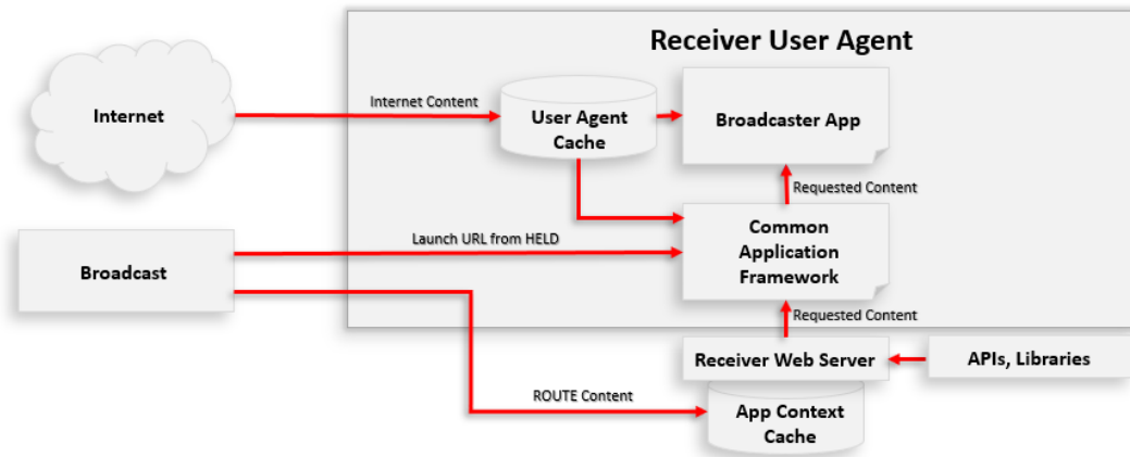
Receiver User Agent Functionality
