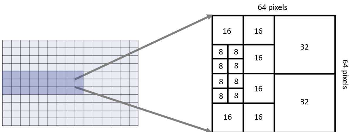
Processing Tiles Containing 64 Pixel Square Coding Tree Units
